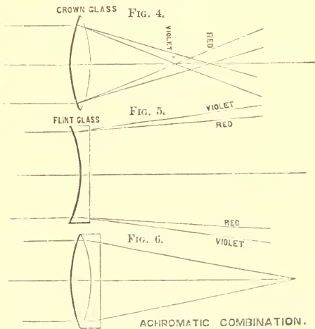
Refraction and Dispersion by Lenses.
